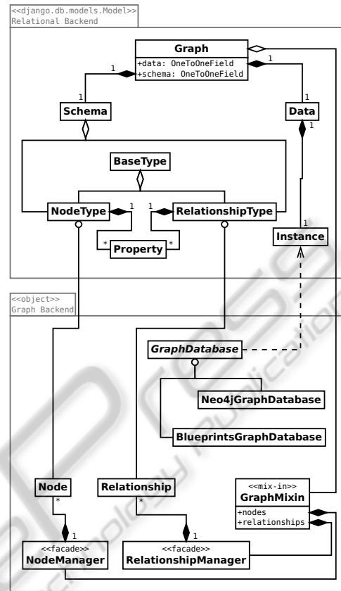
Figure 2: Simplified UML Diagram.
