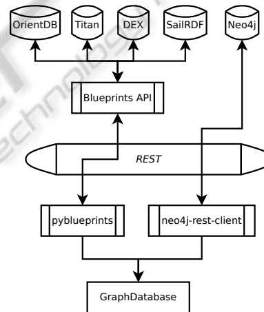
Figure 3: Polyglot graph backend diagram.
